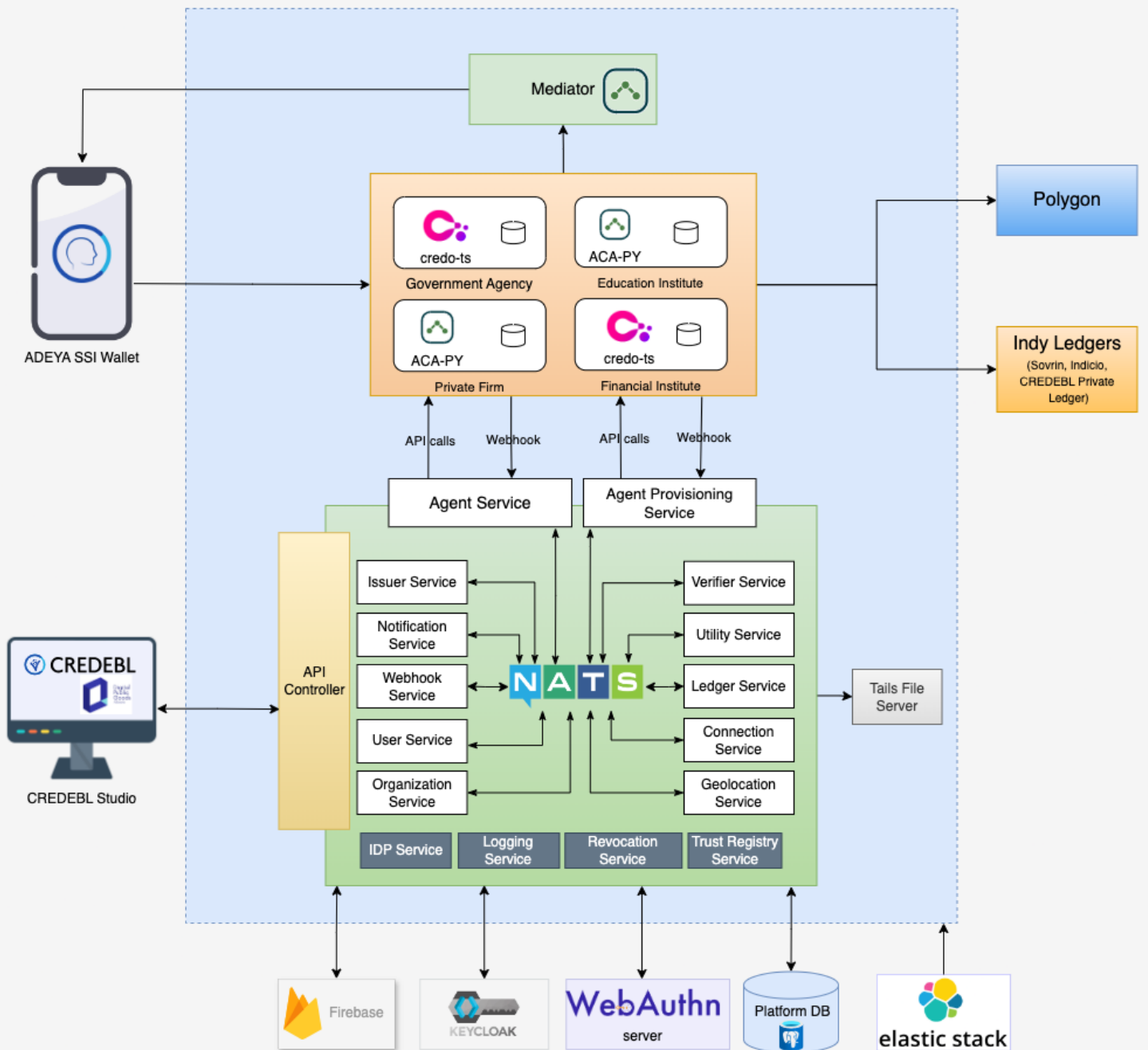
CREDEBL OSS Architecture
